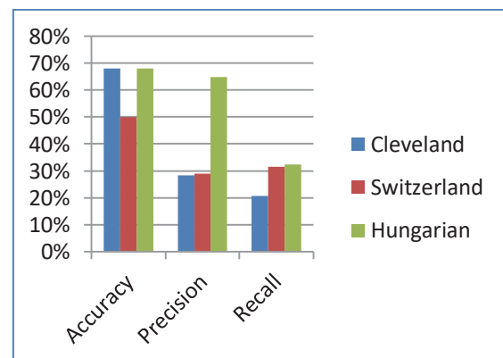
Fig 1: Graph for Performance Measures of Raw Data using KNN classifiers
