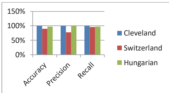
Fig 5: Graph for Performance Measures of Naïve Bayes Classifiers with Min-Max Normalization
