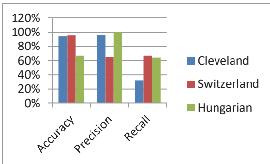
Fig 2: Graph for Performance Measures of KNN Classifiers with Min-Max Normalization
