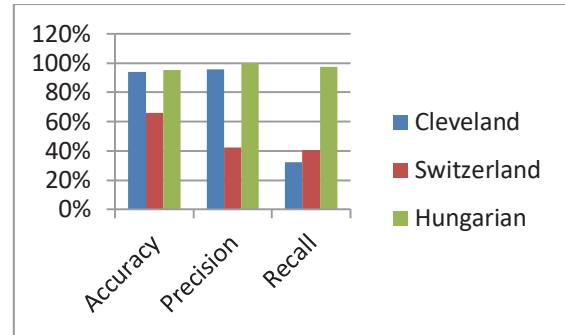
Fig 3: Graph for Performance Measures of KNN Classifiers with Z-Score Normalization
