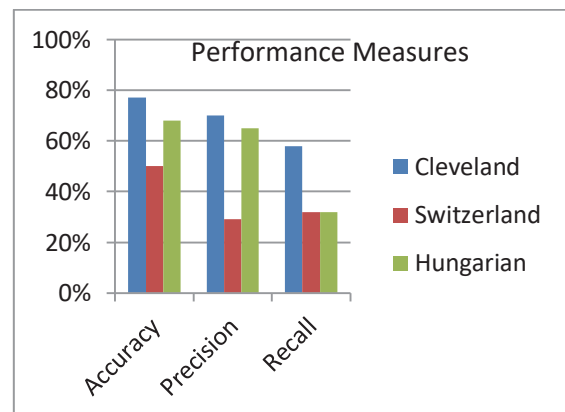
Fig 4: Graph for Performance measures of Naïve Bayes for Raw Data
