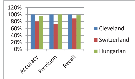
Fig 6: Graph for Performance Measures of Naïve Bayes Classifiers with Z-Score Normalization
